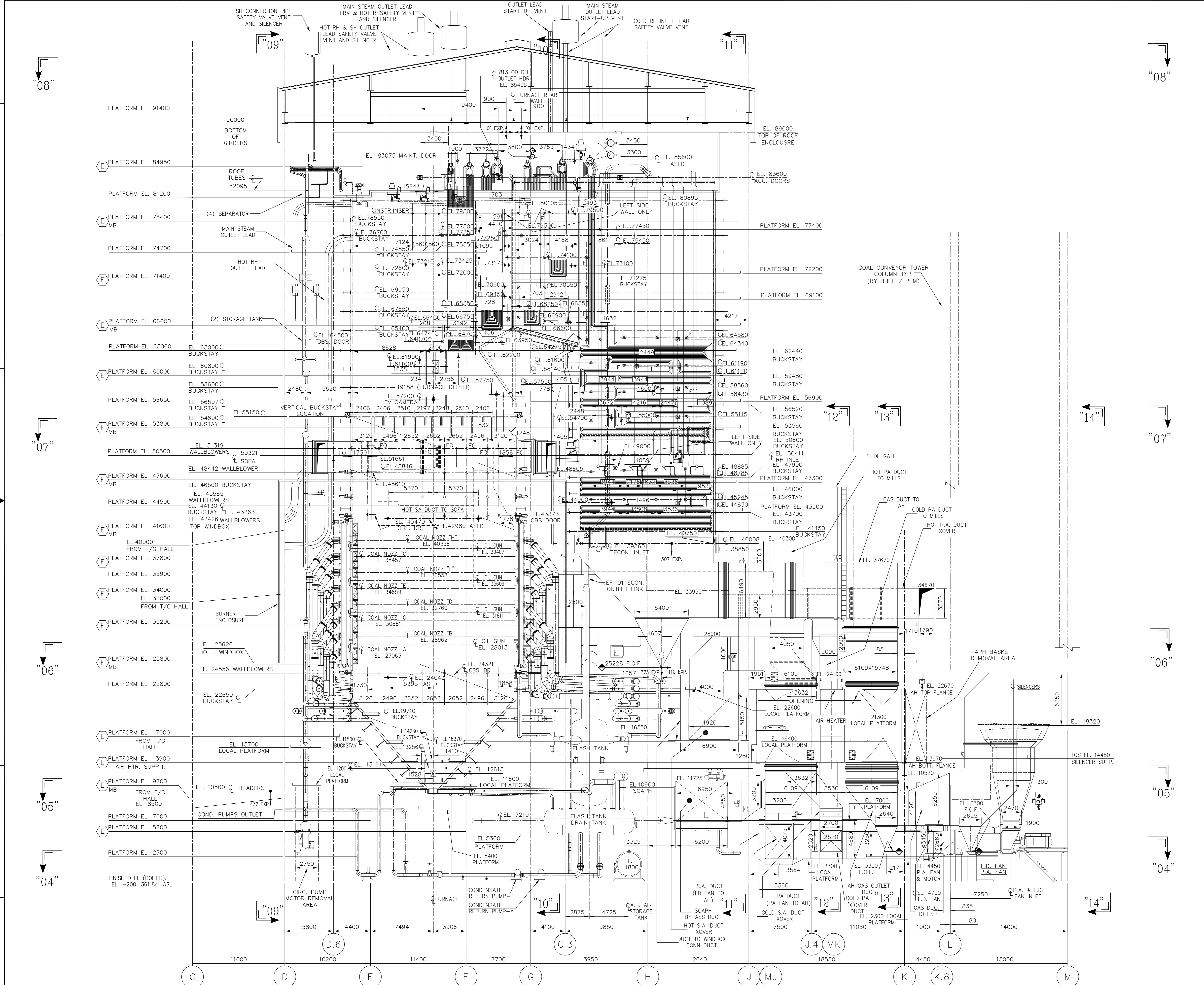
SIDE ELEVATION "02-02" (SEE 00310-1E0001, (B-7))
