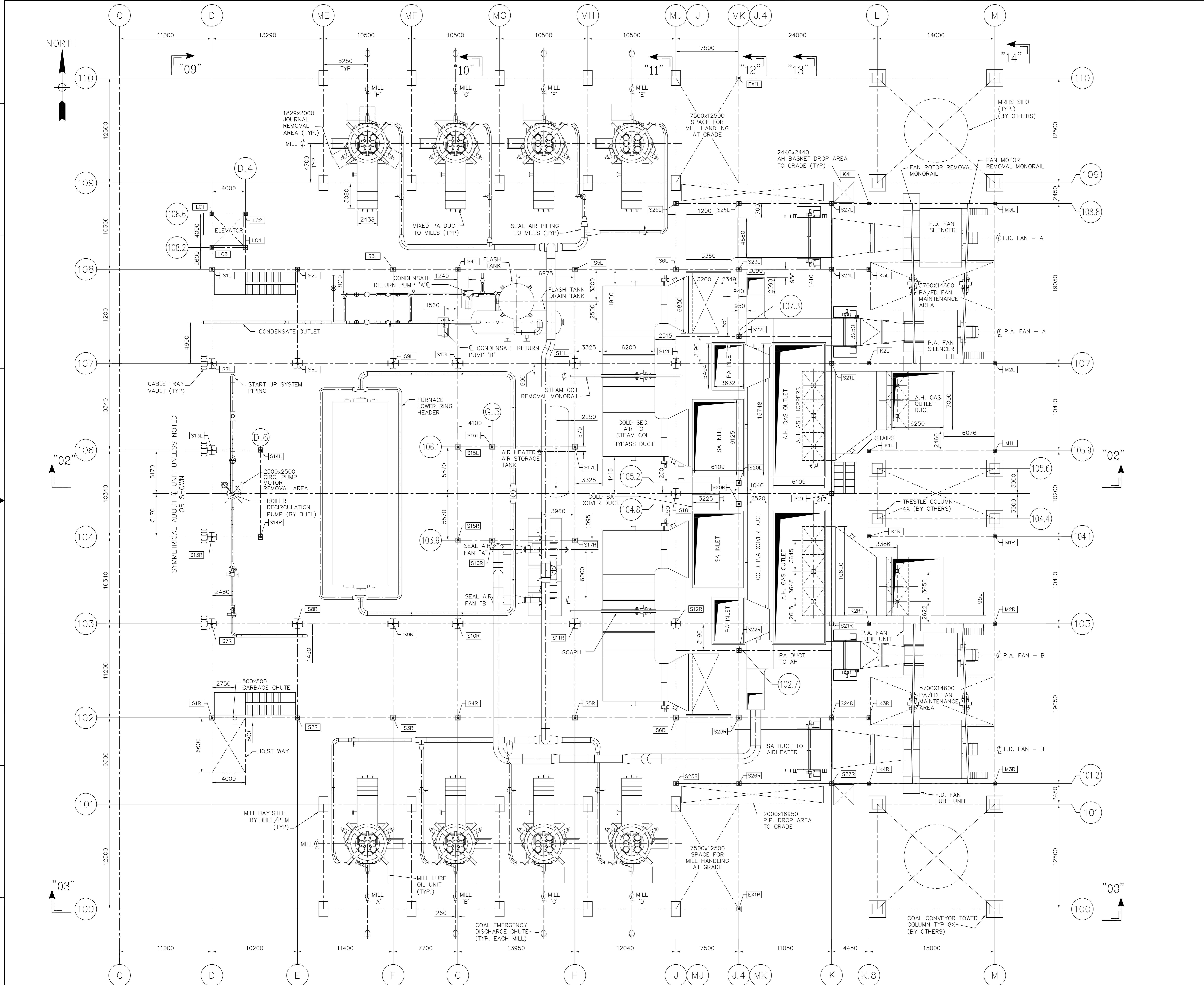
PLAN VIEW "05-05" (SEE 00310-1E0002, (B-8))
