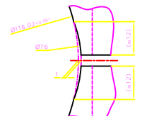
DETAIL - 1 SCALE 5:1
