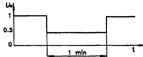
FIG. E3 VOLTAGE DIPS OF \Delta U = 50 PERCENT
