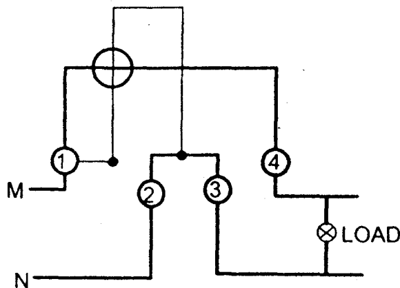
FIG. B SINGLE PHASE TWO WIRE METER SYMMETRICAL CONNECTIONS
