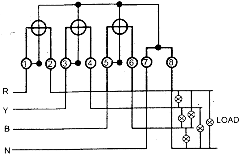
FIG. E THREE PHASE FOUR WIRE SINGLE TARIFF METER FOR DIRECT CONNECTION
