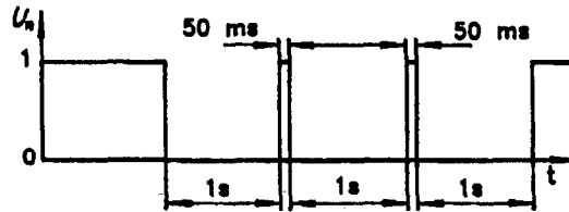
FIG. E1 VOLTAGE INTERRUPTIONS OF \Delta U = 100 PERCENT, 1 s
