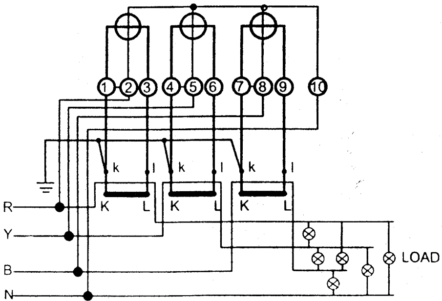
FIG. F THREE PHASE FOUR WIRE METER WITH CURRENT TRANSFORMERS
