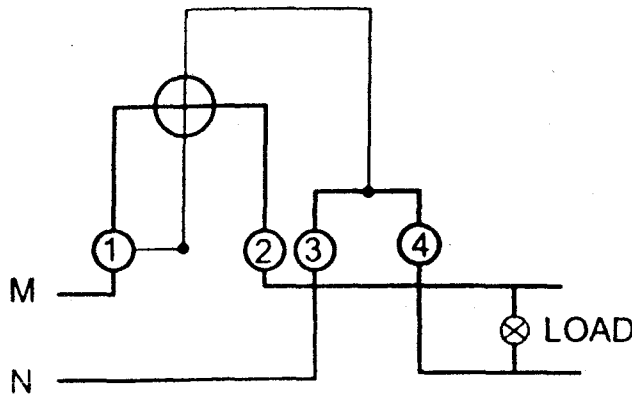
FIG. A SINGLE PHASE TWO WIRE METER
