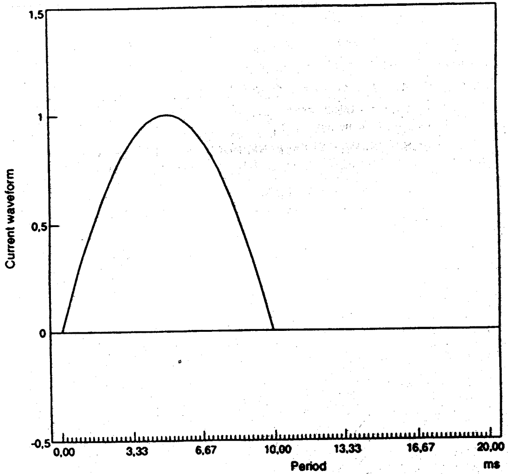
DC and even harmonic test
