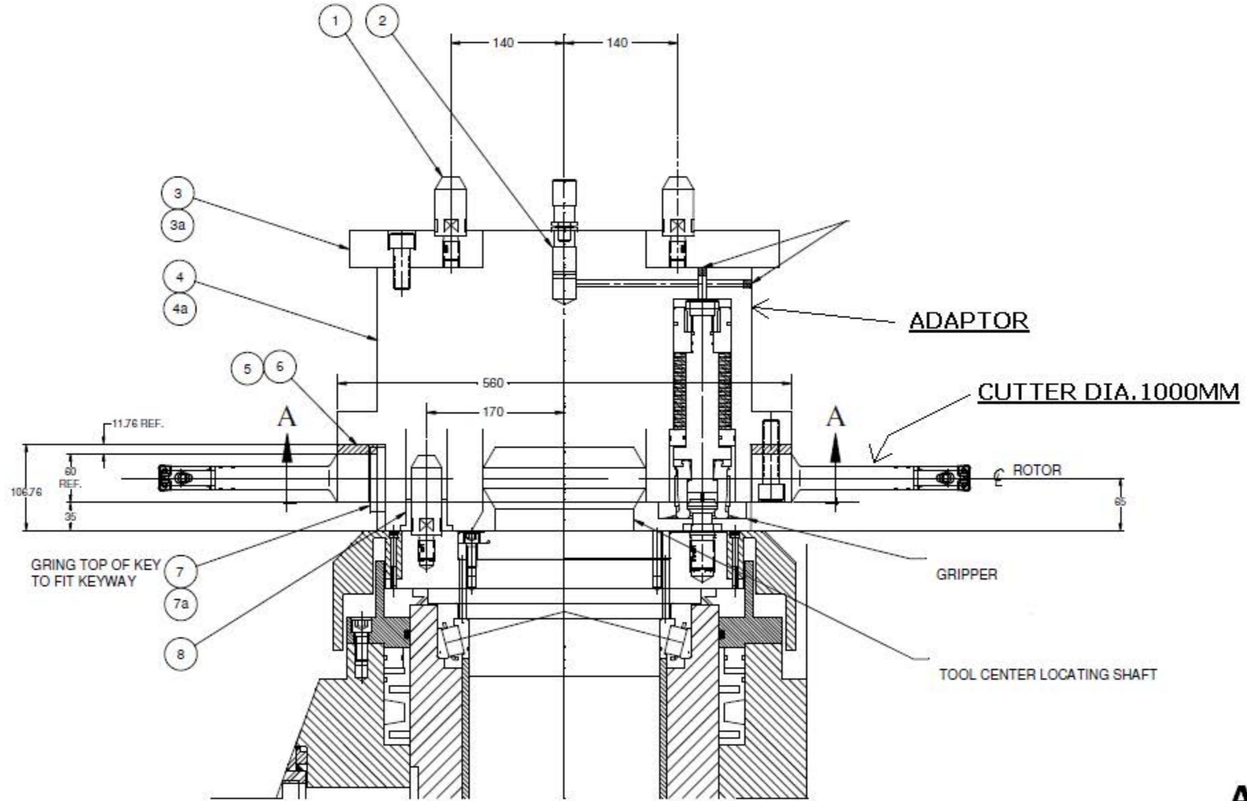
ASSEMBLY OF DIA. 1000MM CUTTER ON ADAPTOR
