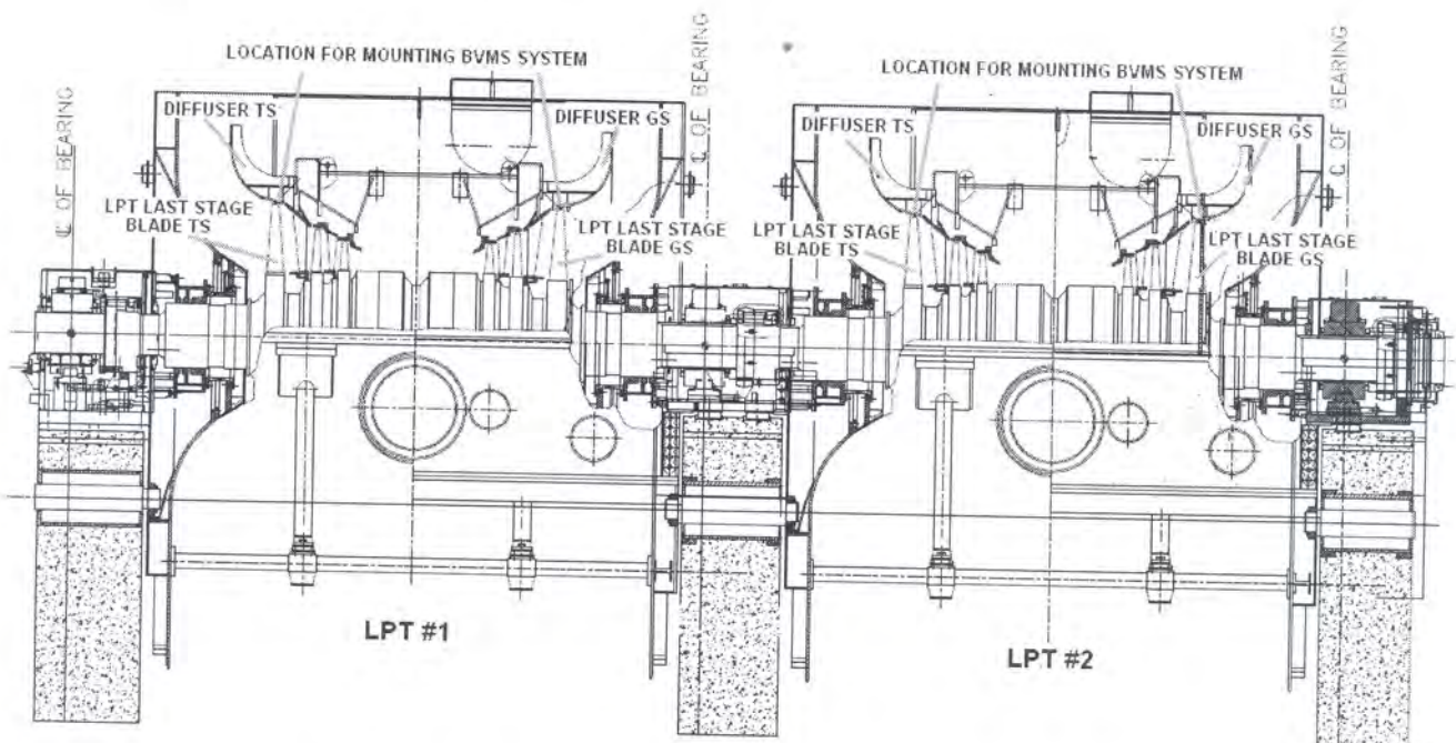
LPT for 600MW showing the desired sensor location
