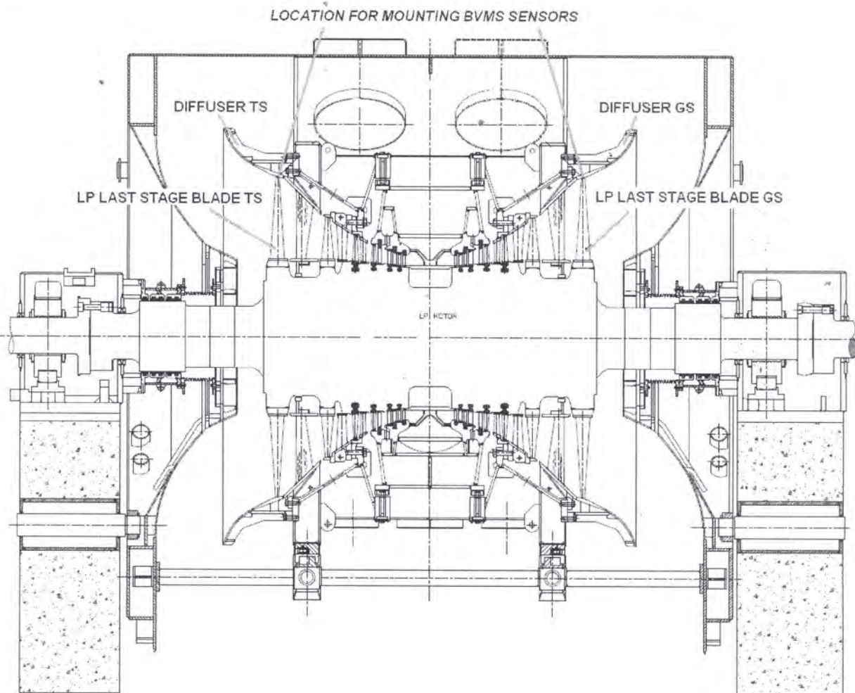
LPT for 250MW showing the desired sensor location
