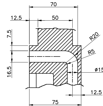
SECTION- 'XX'
