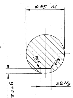
SECTION-CD SCALE:- 1:2.5
