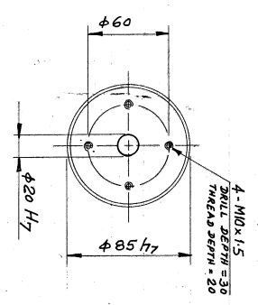
VIEW-E SCALE:- 1:2.5
