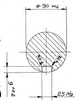
SECTION-AB SCALE:- 1:2.5
