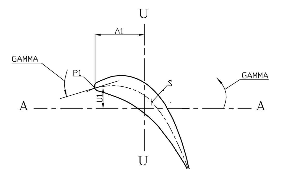
DIMENSIONS OF INLET EDGE
