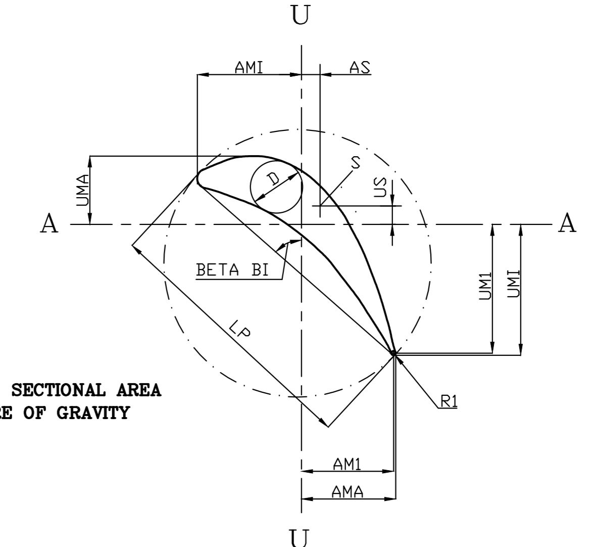
SCHEME OF PROFILE DIMENSION
