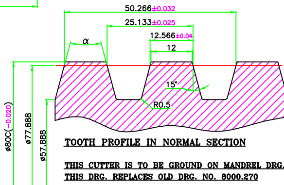
SECTION X-X
