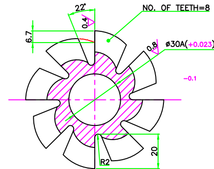
SECTION X-X
