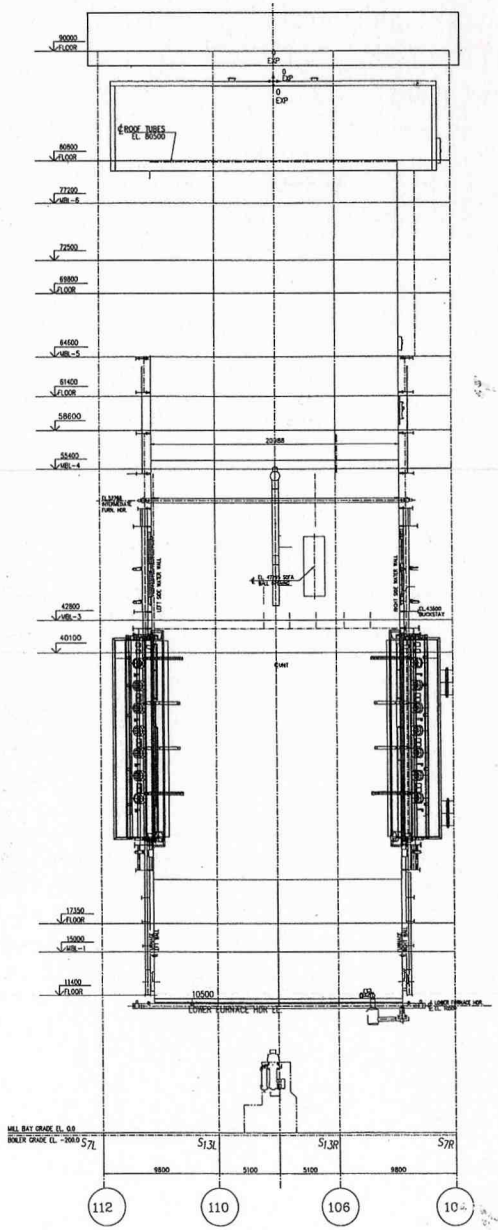
FRONT ELEVATION
