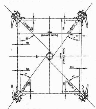
PLAN VIEW OF FLAME MONITORING SYSTEM
