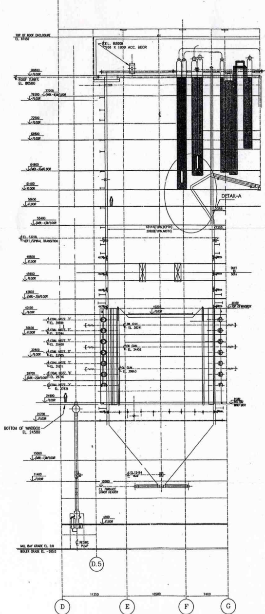
SECTIONAL SIDE ELEVATION
