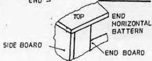
DETAIL - B
