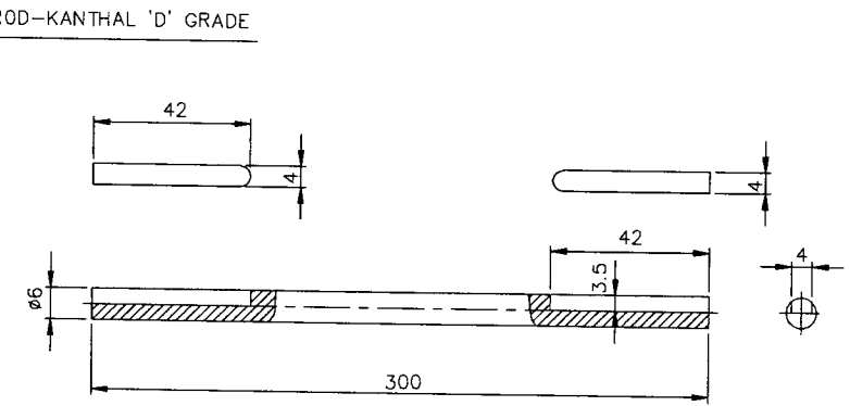
DETAILS OF TERMINAL ROD
