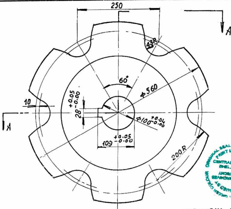
VIEW FROM A-A
