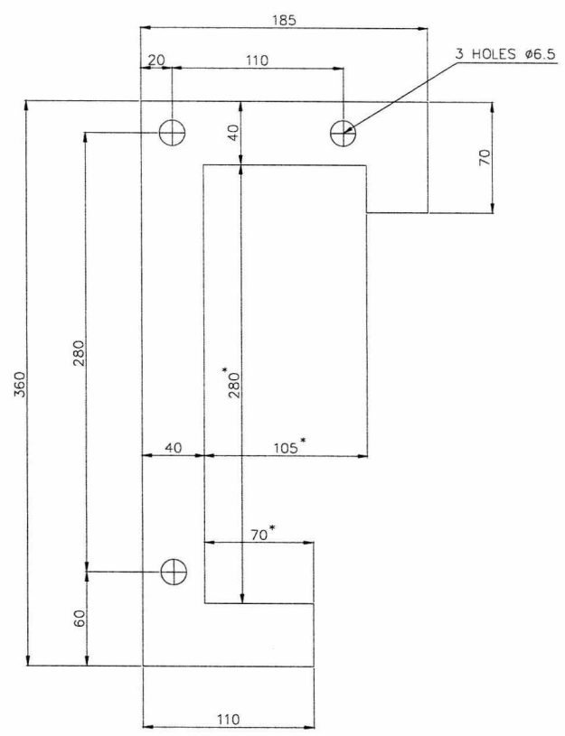
VIEW - A (END PLATE DETAILS)
