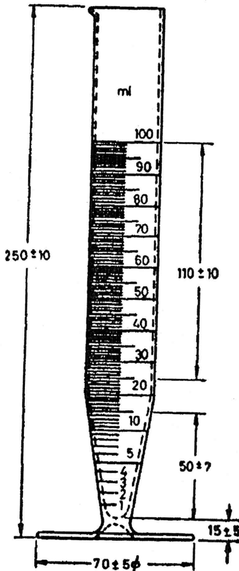
FIG. 6 RECEIVER
