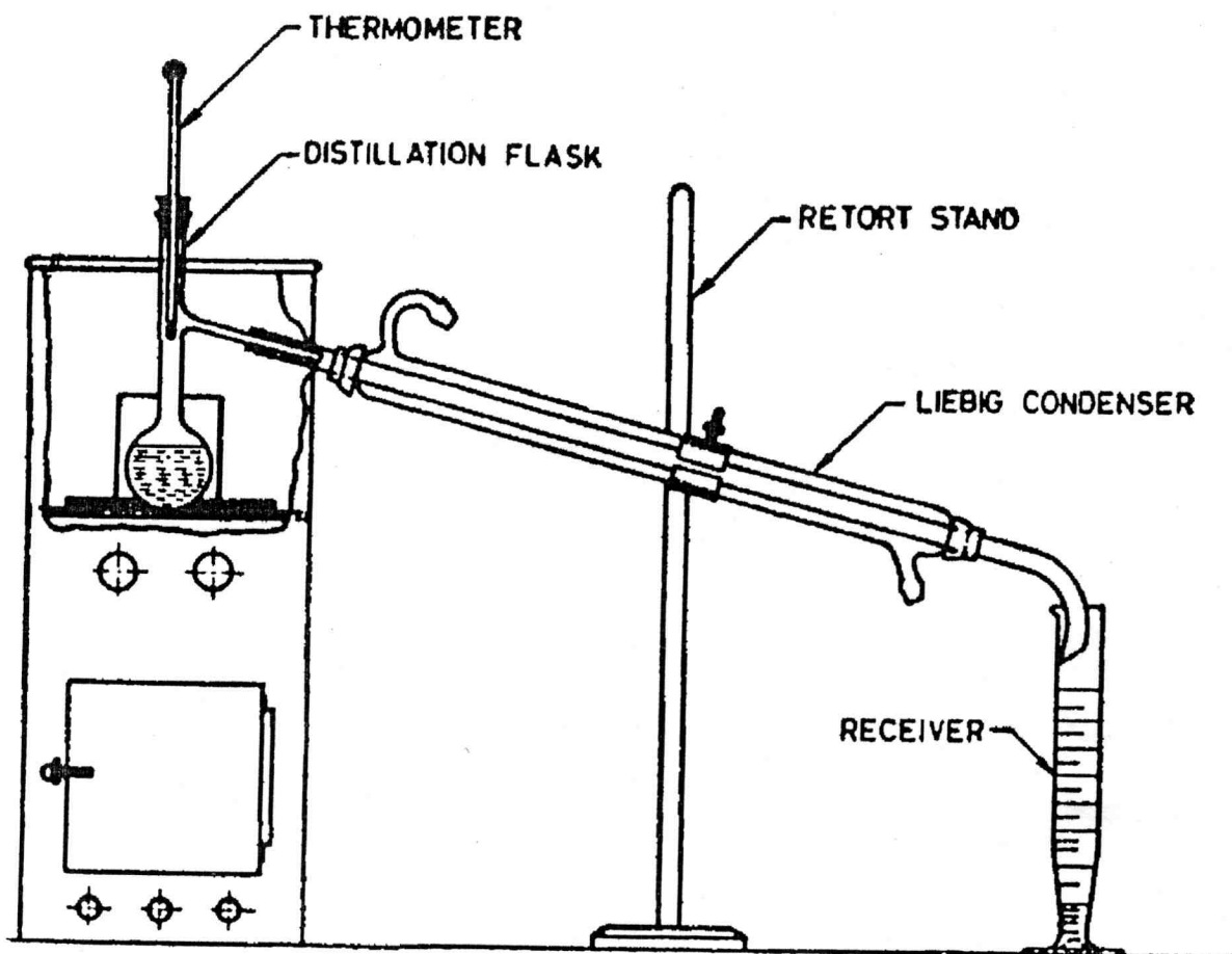
FIG. 7 ASSEMBLY OF APPARATUS FOR DETERMINING DISTILLATION RANGE
