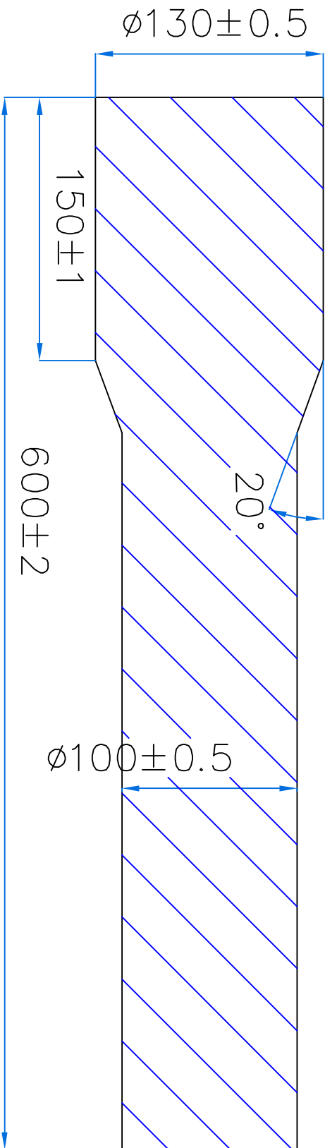
MOVABLE MAIN CONTACT FOR COMPACT GCB
