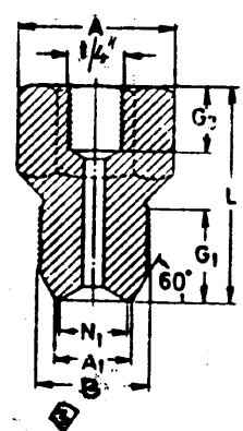
MODEL NO B 03-06 1/2" 03-07 3/4" 03-08 1/8" POS. 04 CONNECTION NIPPLE SIBCO MODEL NO. 03-06/07/08
