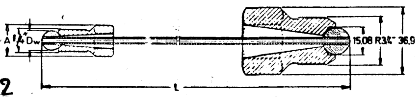
FLEXIBLE HIGH PRESSURE PIPE. SIBCO MODEL NO. 01-02
