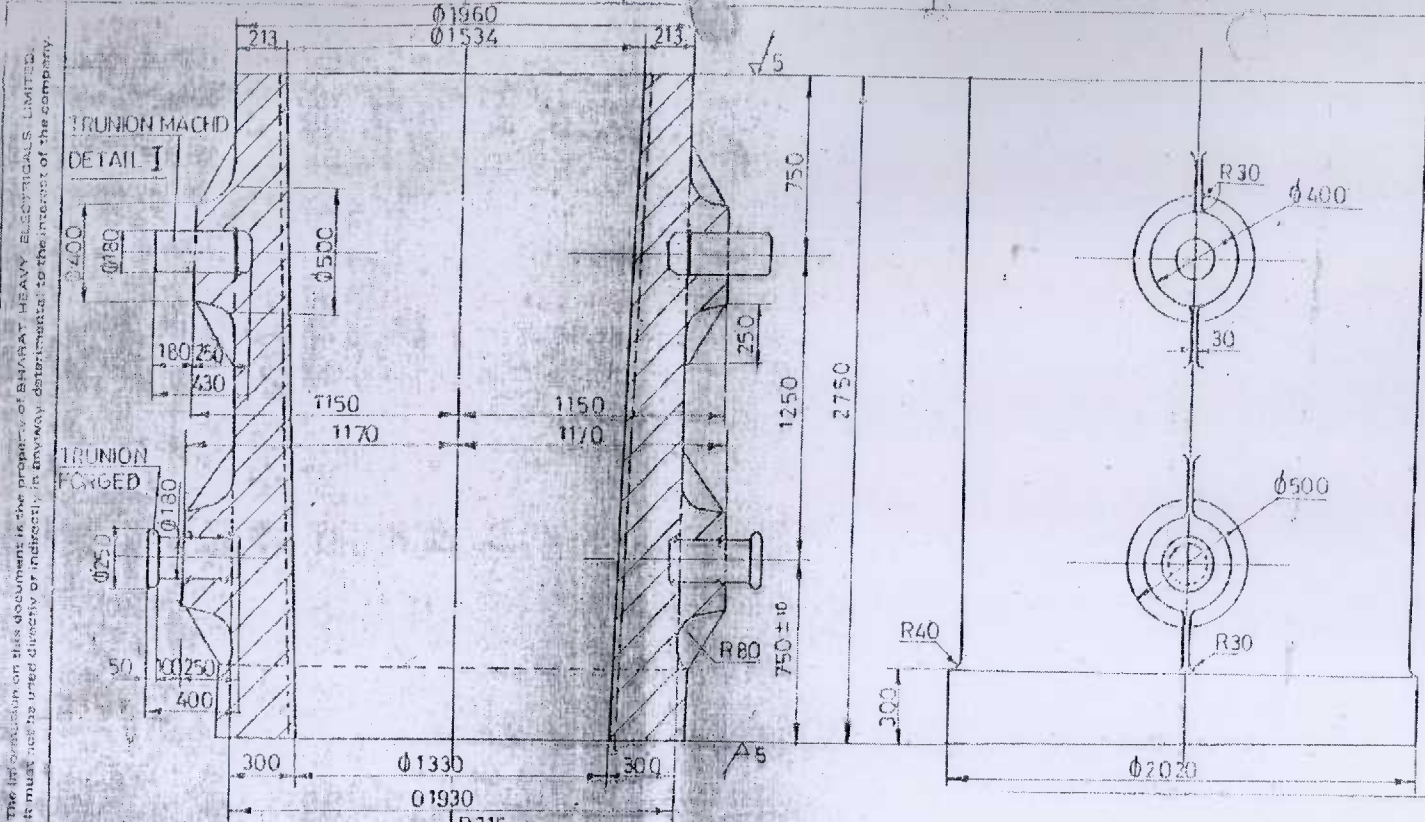
TR UNION MACHD DETAIL I SCALE 1:10
