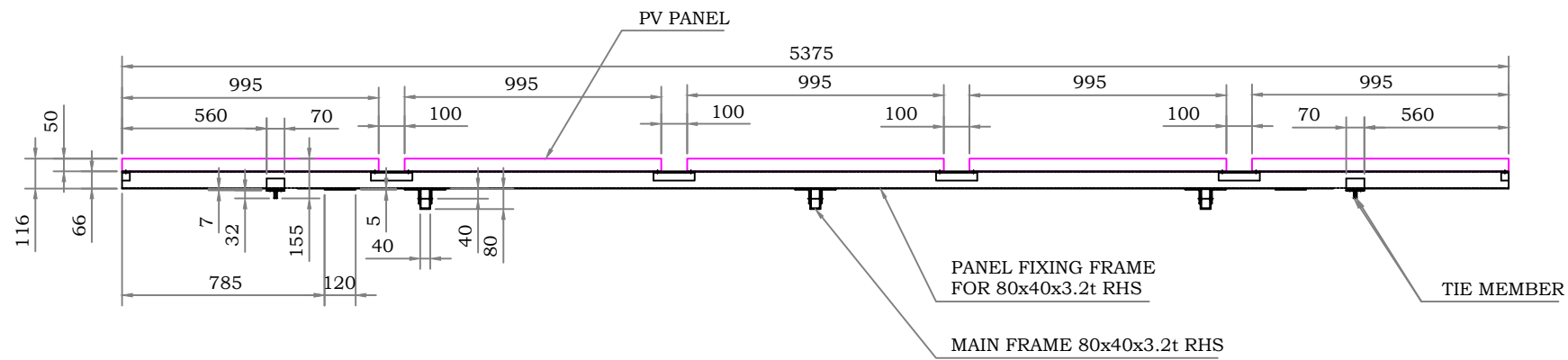
SECTION C-C
