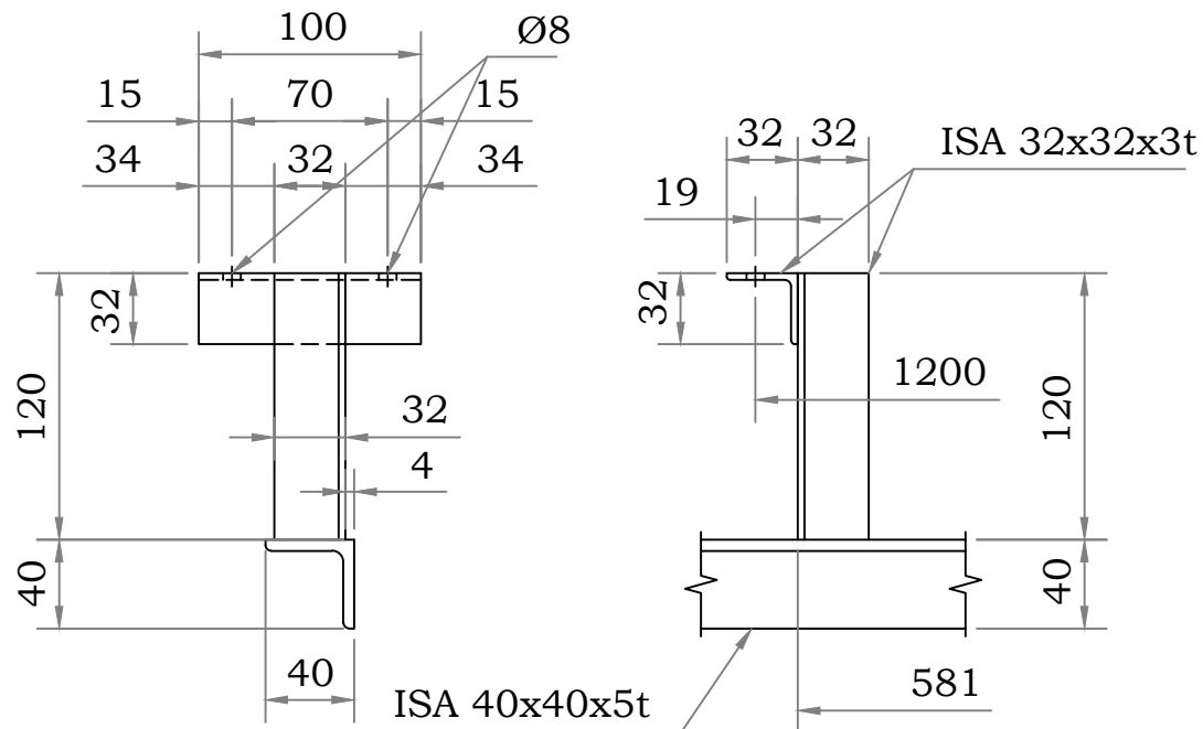
DETAIL - K
