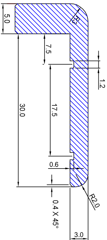
DETAIL A
