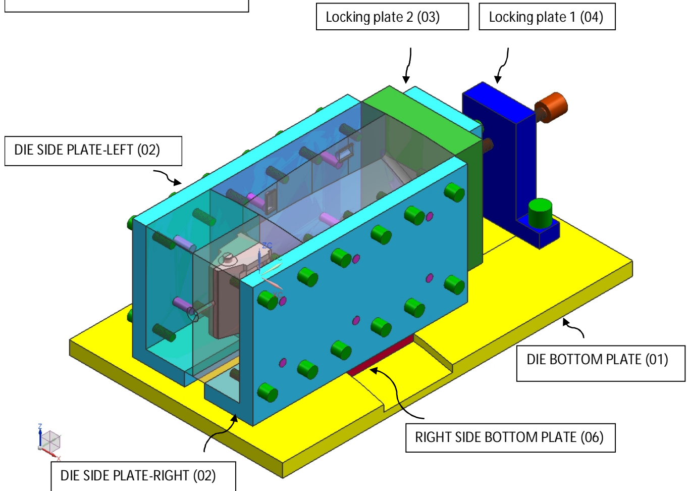
FIGURE: DIE ASSEMBLY FOR FRAME-05 STAGE-02 GT BUCKET
