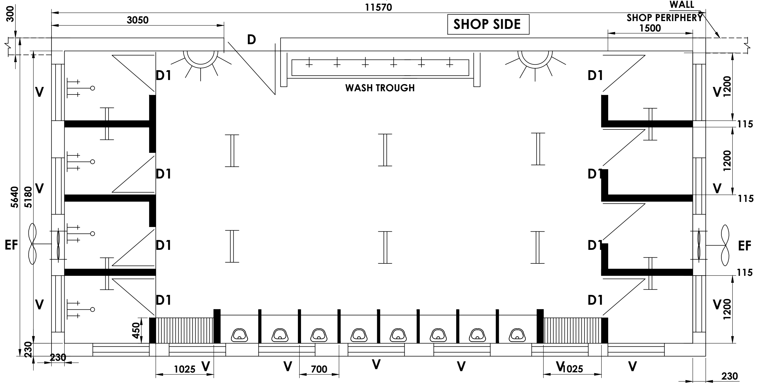
GENERAL ARRANGEMENT OF TOILET 1 & 2
