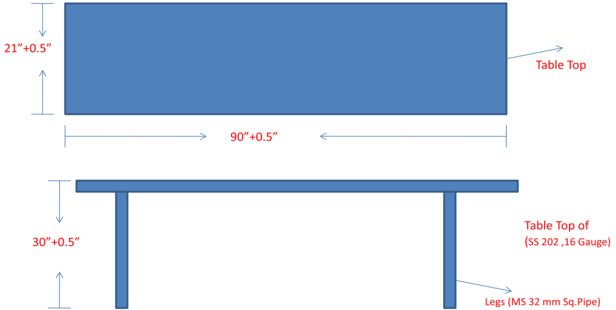
Fig .2 Typical Dimension of dining table
