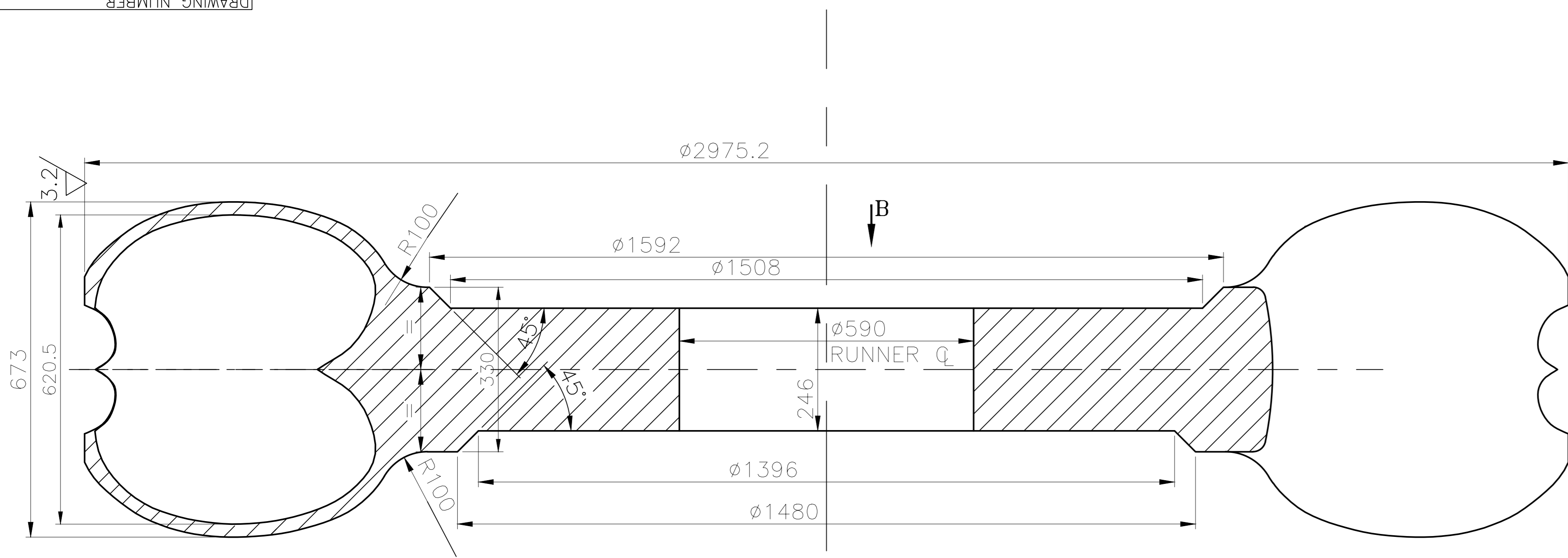
SECTION-AA
