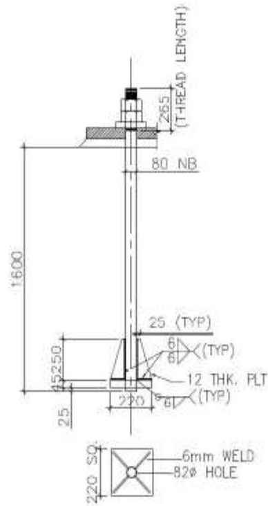
TYP DETAIL OF ANCHOR BOLT
