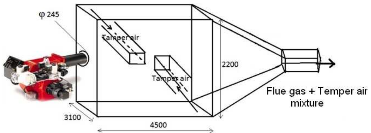
Figure: Schematic diagram combustion chamber with oil burner. All dimensions are given in "mm" and drawn not according to scale.
