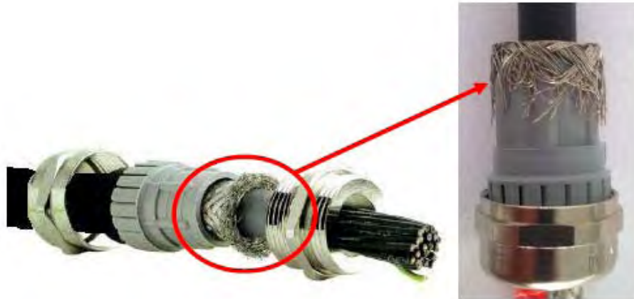
Figure 3 – Shield connection
