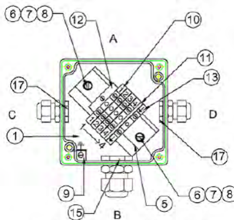
Figure 4 – Connection boxes internal view
