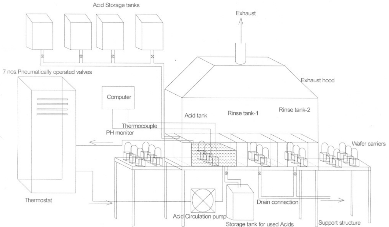
Schematic of Acid texturisation system for mc-Si wafers: Linear movement
