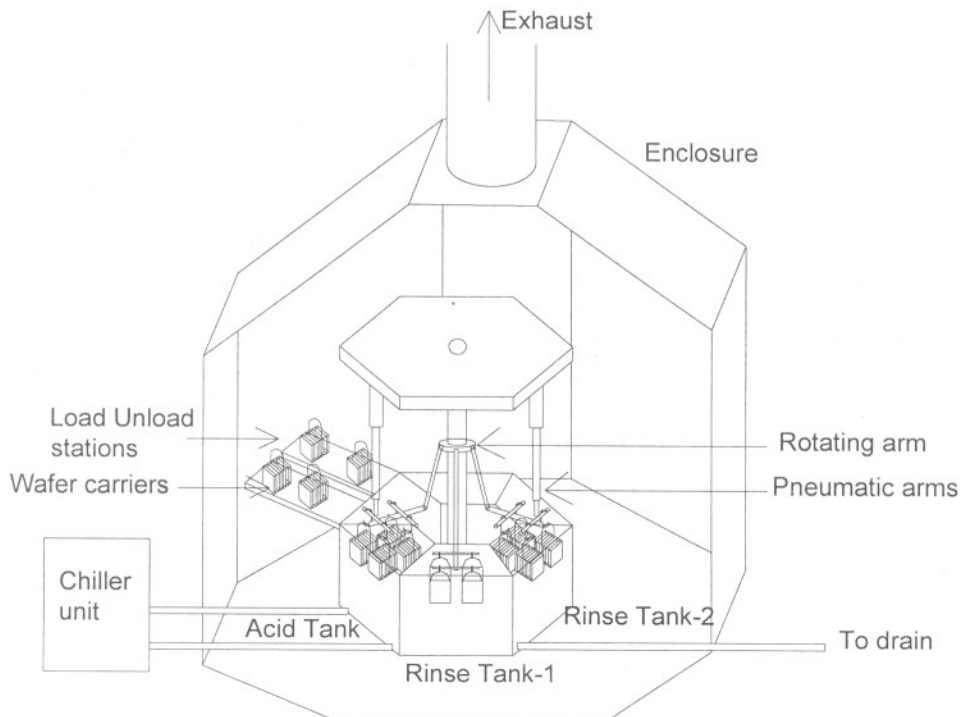
Schematic of Acid Texturisation System for mc-Si Wafers: Circular movement
