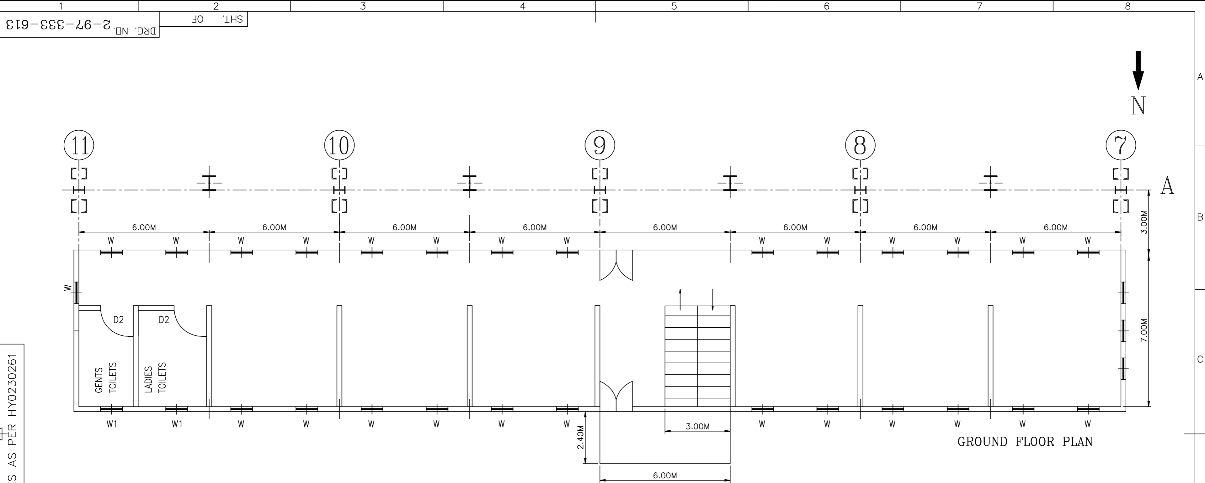
G.T.MACHINE SHOP ANNEXE IN TWO FLOORS : 7x48.0M
