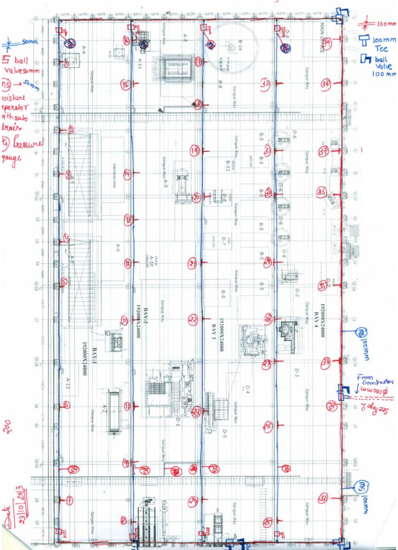
Layout plan of pipe line distribution inside Fabrication Plant
