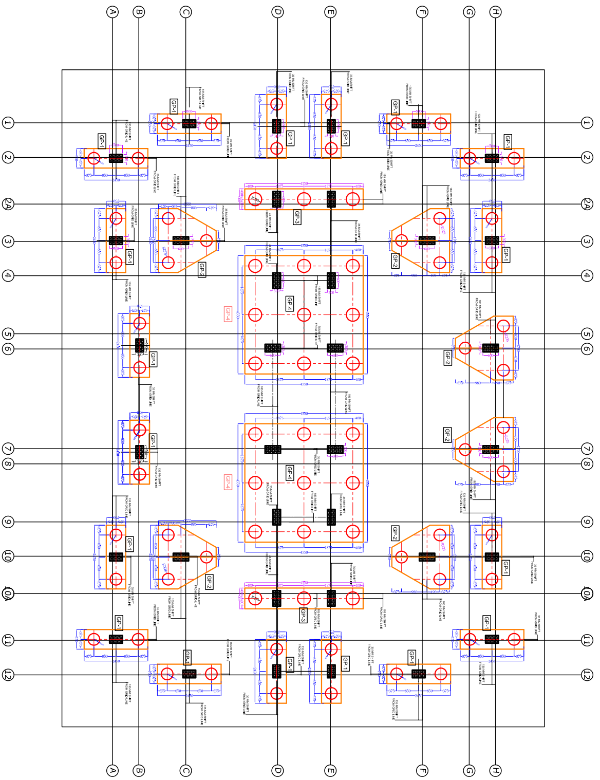
TYPICAL PILE LAY - OUT PLAN (FOR MULTI STORED BLOCKS)
