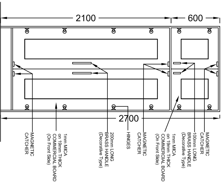
CUBOARD DETAIL (TYPICAL) FOR 'A' & 'B' TYPE
