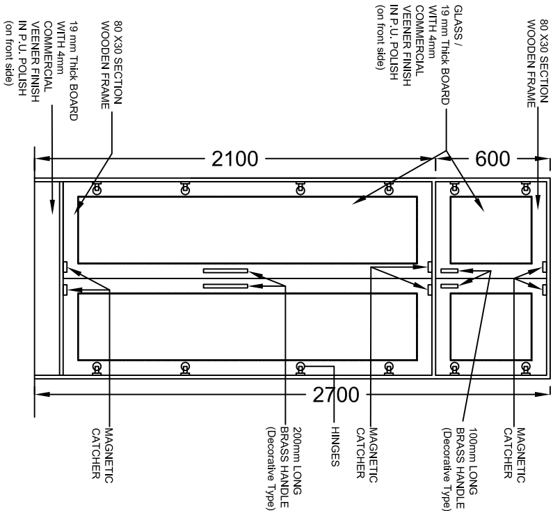
CUBOARD DETAIL (TYPICAL) FOR 'C', 'D', 'CEO' AND OTHER BUILDINGS
