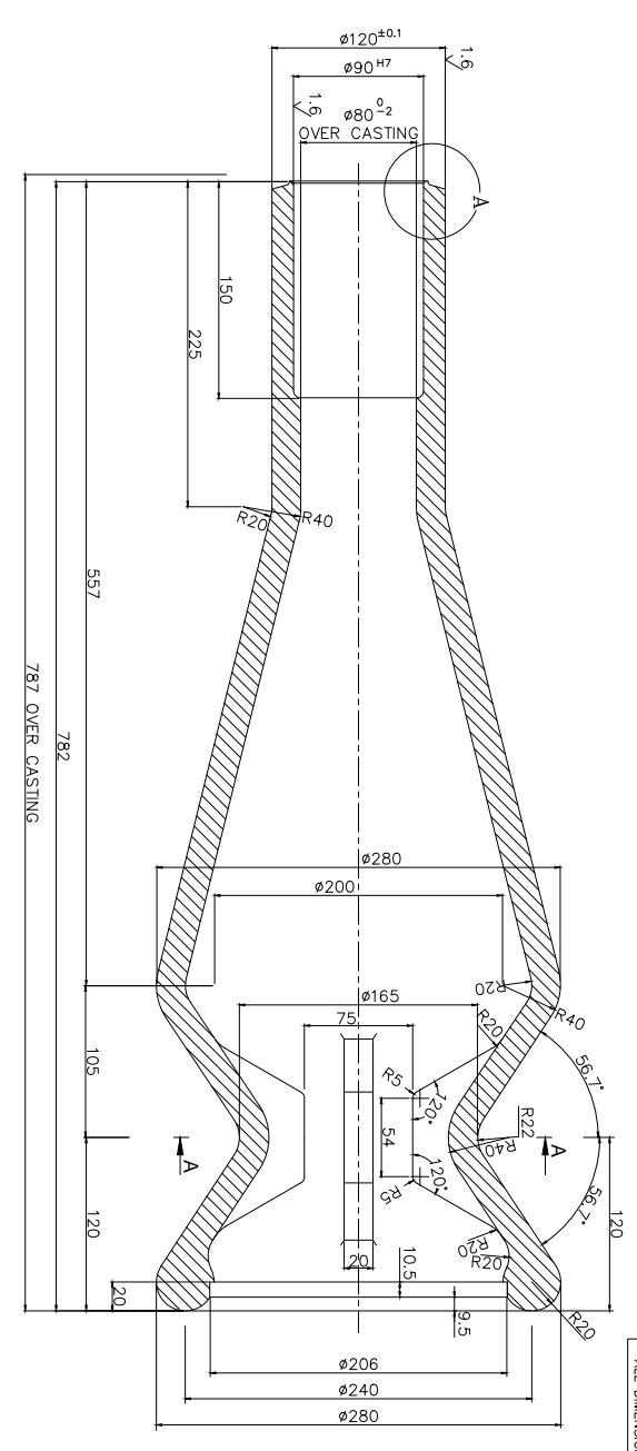
DETAIL OF CHARGE AND DISCHARGE ROLLER MATERIAL - HK ALLOY (25% Cr, 20% Ni.)
