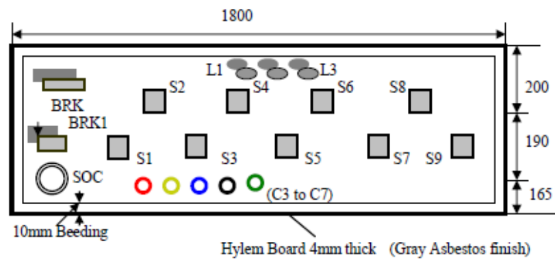
Fig. 2. Electrical Panel Layout.
