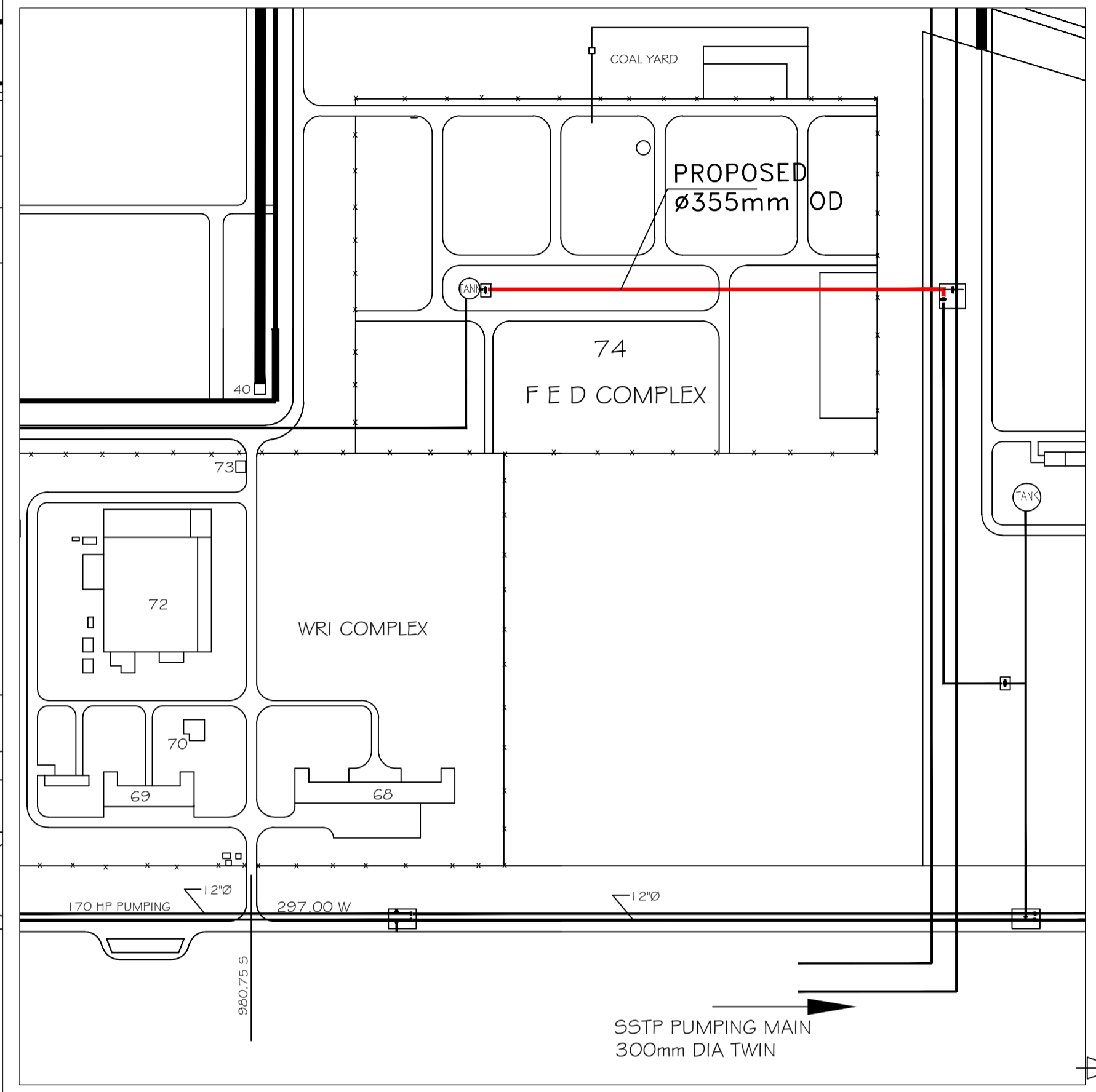
PLAN SHOWING HDPE ROUTING FROM CCDP MAIN TO FCB TANK
