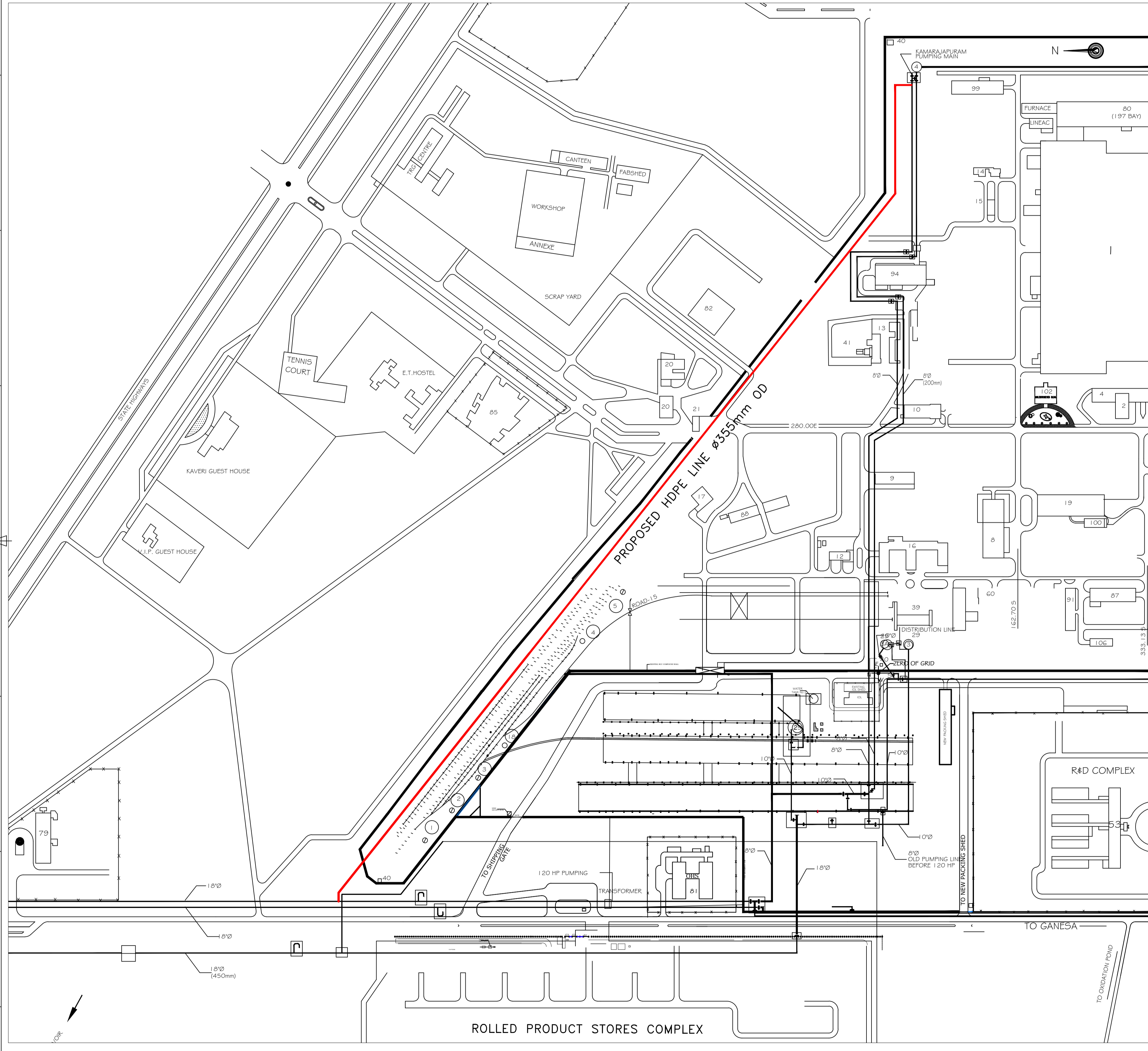
PLAN SHOWING HDPE ROUTING FROM RPS RAILWAY GATE TO TANK 4
