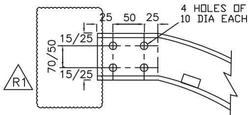
ENLARGED VIEW OF "X"
