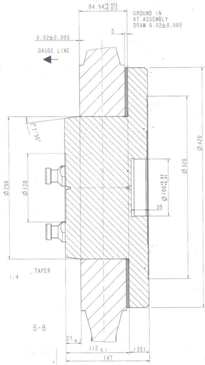
SKETCH OF ADAPTOR FOR REFERENCE
