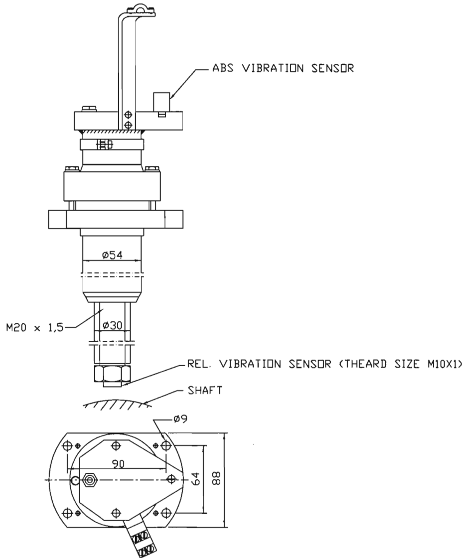
DUAL PROBE HOUSING
