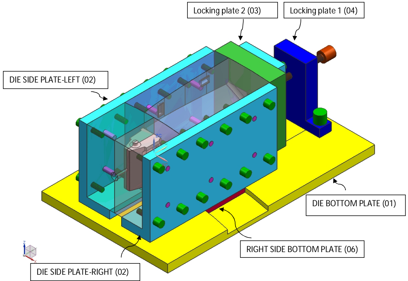
FIGURE: DIE ASSEMBLY FOR FRAME-05 STAGE-02 GT CUTTER TEETH BUCKET
