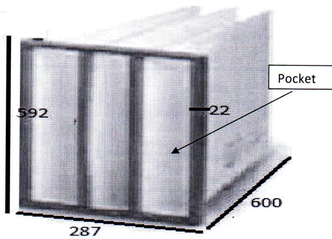
Drawing of pocket filter (All dimensions in mm)
