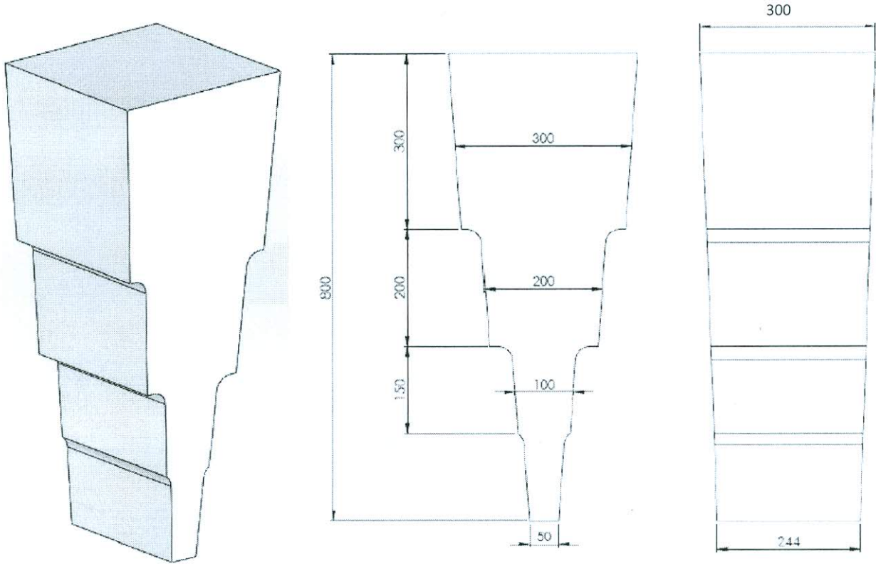
Dimensions of an IN625 Test Block casting
