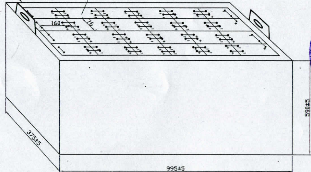
SIMCO F/L 48VOLT BATTERY DRAWING.
