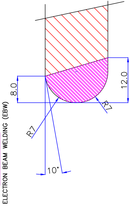
DETAIL 'A'
