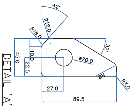
6 No. of PLATES. Material : SS-304L
