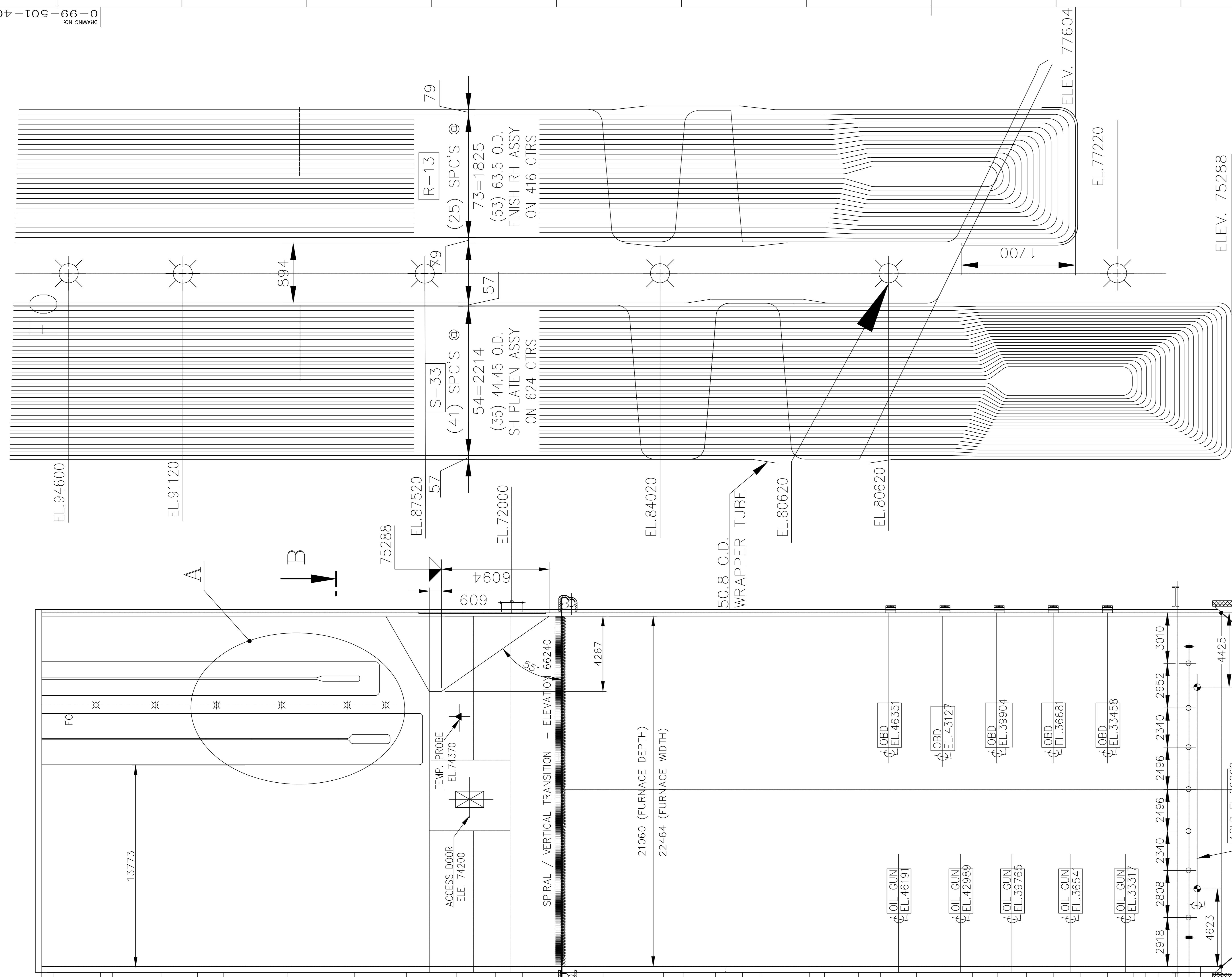
DETAIL-A
