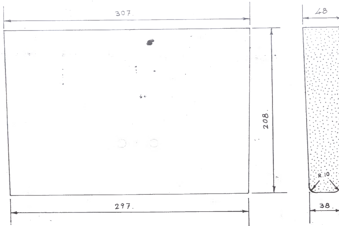
POURING BASIN Drg No: 2-04-476.
