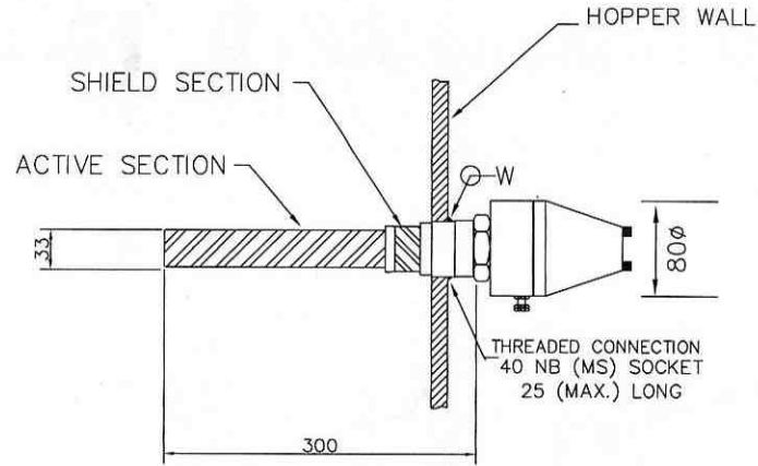
SENSING PROBE ( RIGID )
