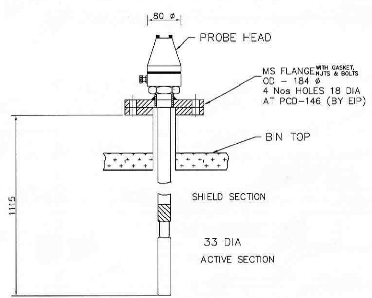
SENSING PROBE
