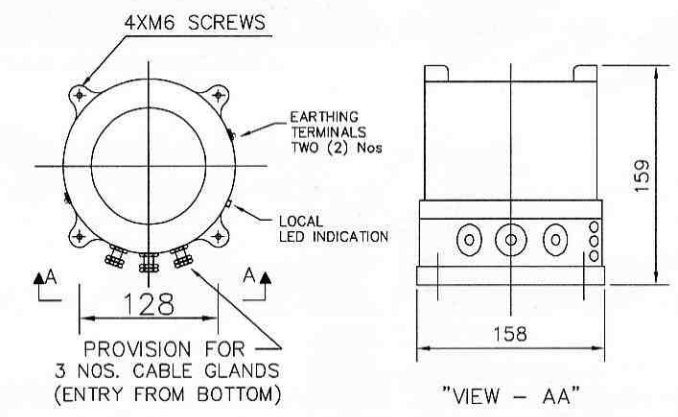
ELECTRONIC CONTROLLER
