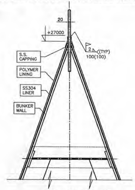
S.S. CAPPING AT TOP OF DISCHARGE HOPPERS
