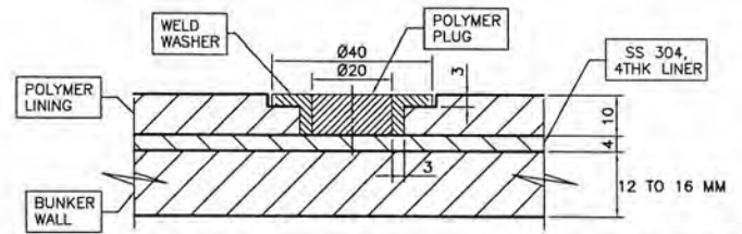
FIXING OF LINER WITH WELD WASHER TYPE FASTENER
