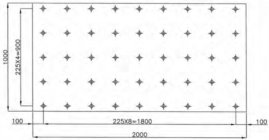
SPACING OF FASTENING POINTS FOR POLYMER LINERS (TYPICAL)
