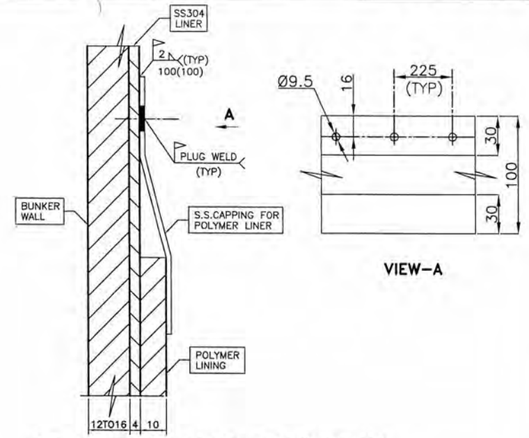
S.S. CAPPING AT LINER TOP (TYPICAL) SHAPE DEPENDS ON ACTUAL LOCATION)
