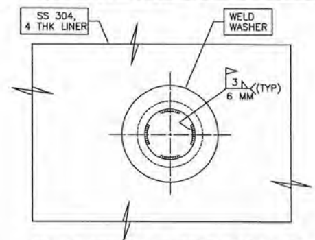
WELD WASHER TYPE FASTENER
