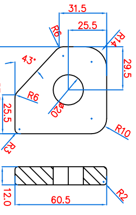
DETAIL 'C' 16 No., SS-304L
